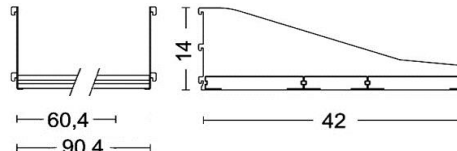
Shelves 2630.D1/D2
