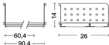
Shelves 2630.B1/B2
