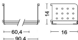
Shelves 2630.A1/A2
