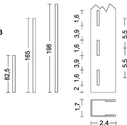
Uprights 2630.H1/H2/H3
