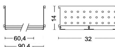
Shelves 2630.C1/C2
